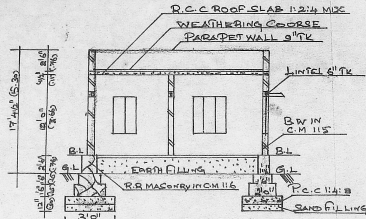
SECTION ON 'DM'
